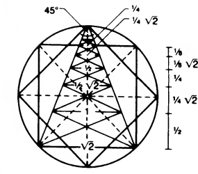
① \pi/4 triangle (according to A. V. Drach)
